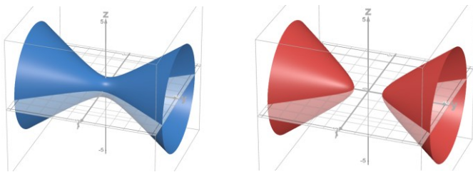
Images: 1-sheated vs 2-sheated hyperbola.
